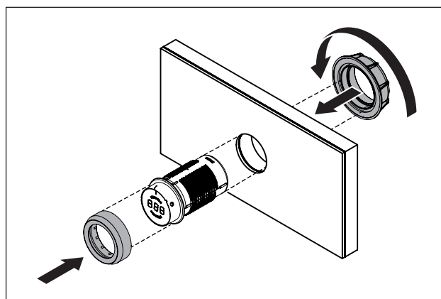
Fig. 5.14 Installing the control knob
