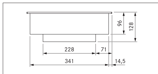
Fig. 3.3 PKIW1 Device dimensions front view
