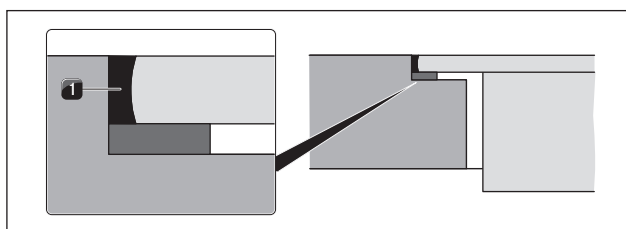
Fig. 5.20 Silicone sealant with flush installation
