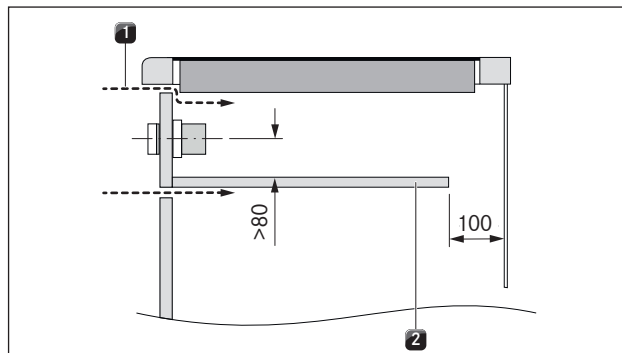
Fig. 5.8 Air supply via the front area
