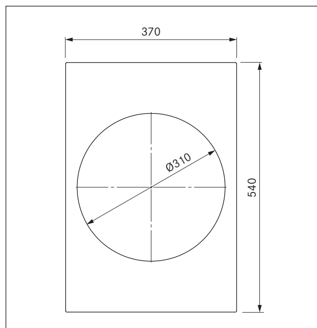
Fig. 3.2 PKIW1 Device dimensions aerial view
