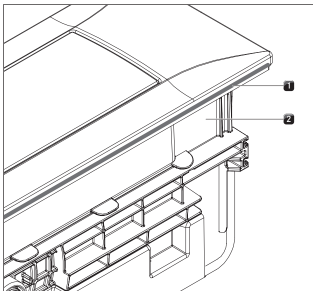
Fig. 5.7 Removing the plastic strip from the side of the cooktop extractor
