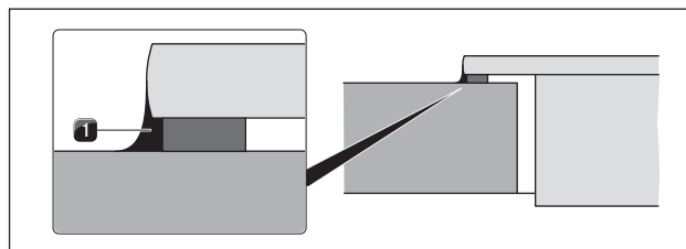
Fig. 5.21 Silicone sealant with surface mounting
