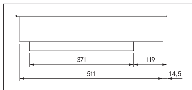
Fig. 3.4 PKIW1 Device dimensions side view
