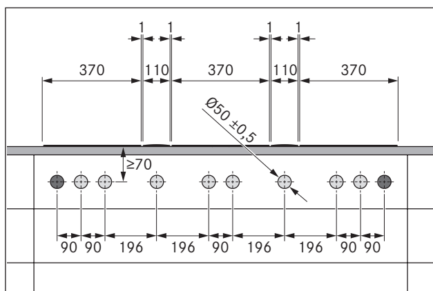
Fig. 5.16 Bore holes for 3 cooktops and 2 extractors
