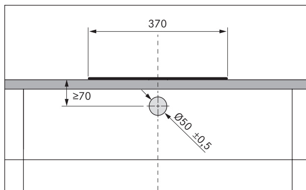
Fig. 5.13 Drilling diagram
