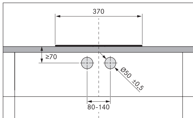
Fig. 5.11 Drilling diagram
