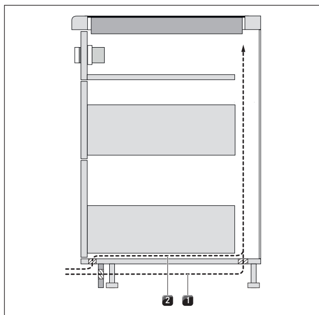
Fig. 5.9 Air supply via the plinth area
